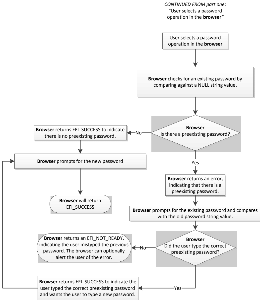
Figure 122. Password Flowchart (part two)
