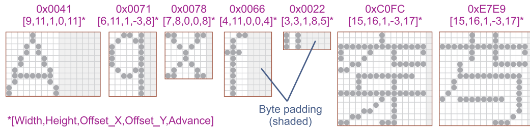
Figure 96. Proportional Font Parameters and Byte Padding
