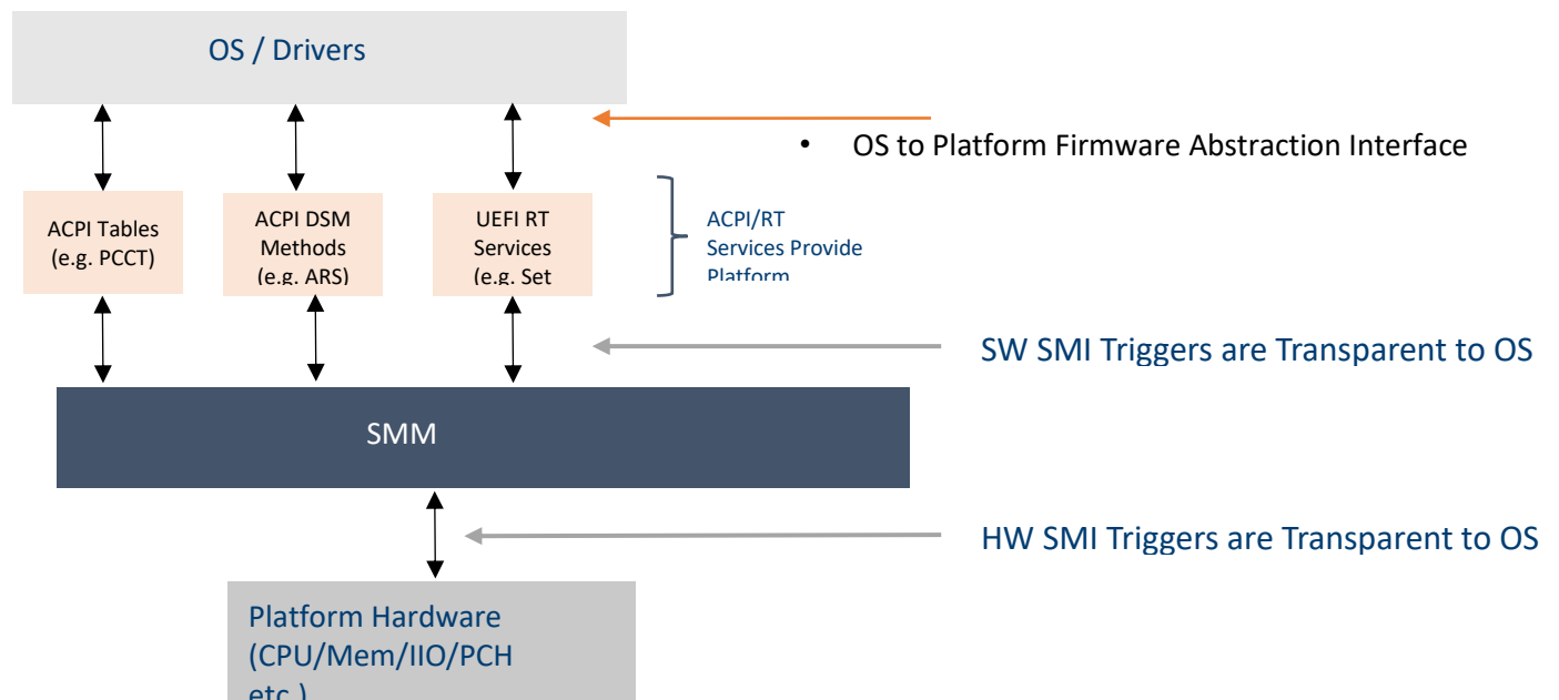
Figure 2-1 SMI Triggers
