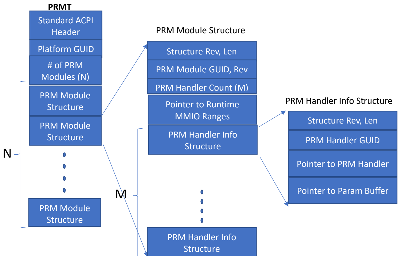
Figure 3-2 PRMT Topology
