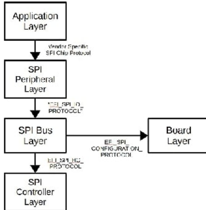
Fig. 18.2: SPI Layers
