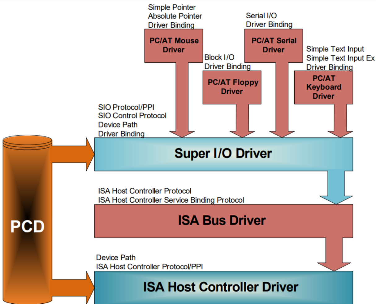
Fig. 14.1: Super I/O and ISA Host Controller Interactions
